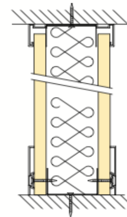
Full height solid
