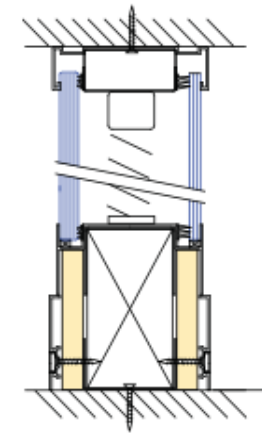
Full height double glazed with venetian blinds
