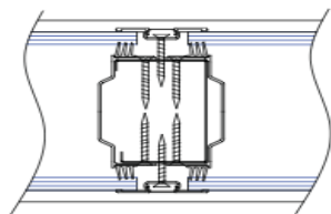
Double glazed mullion
