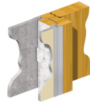
Timber door frame to solid wall
