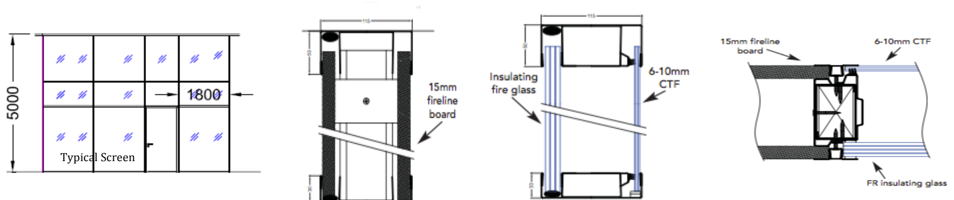
Double glazed vertical section
